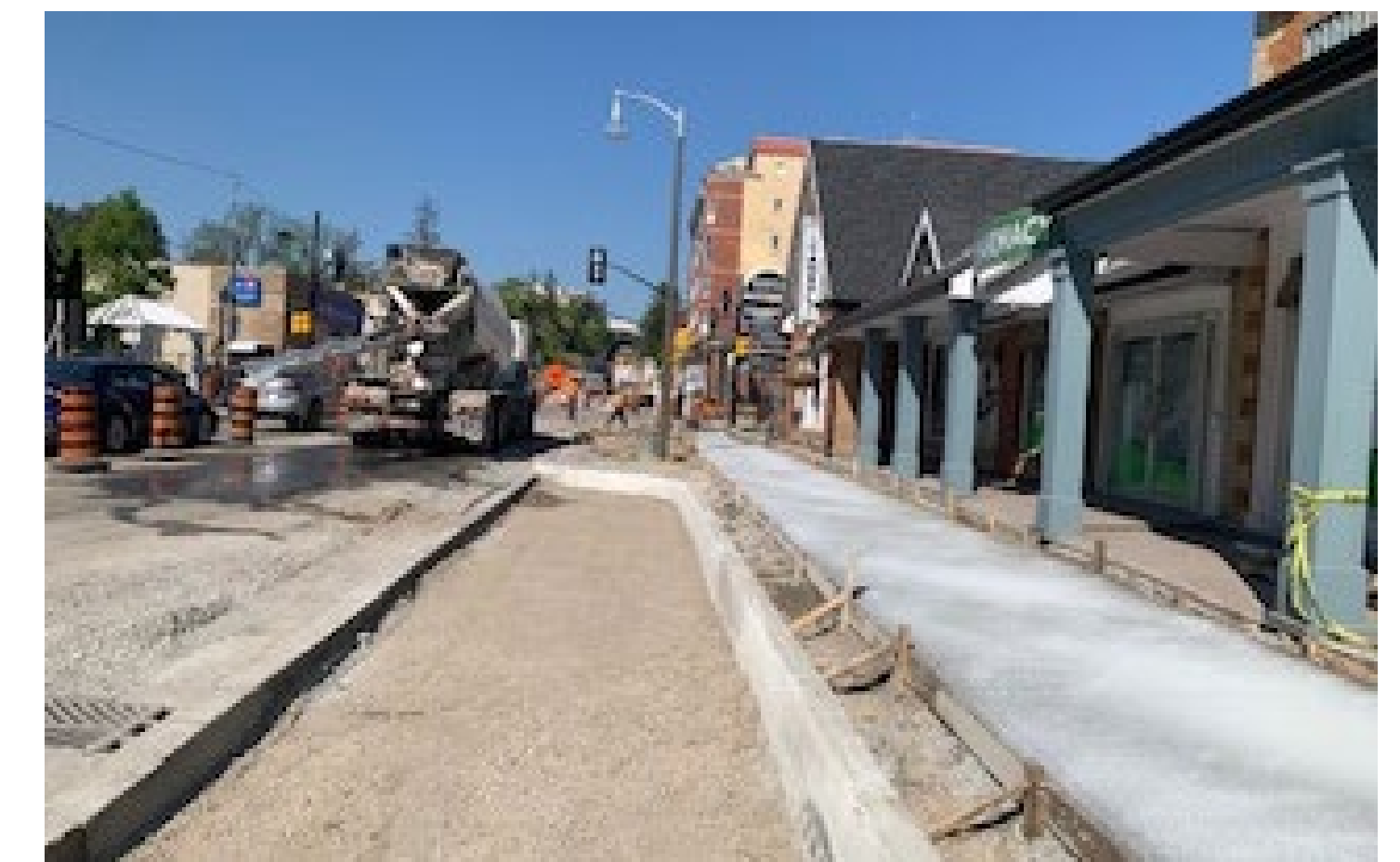
Typical streetscaping construction of curb and sidewalk
